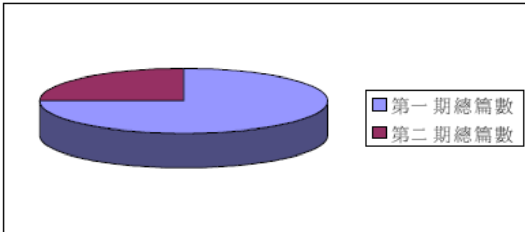
Fig 1. Statistics
